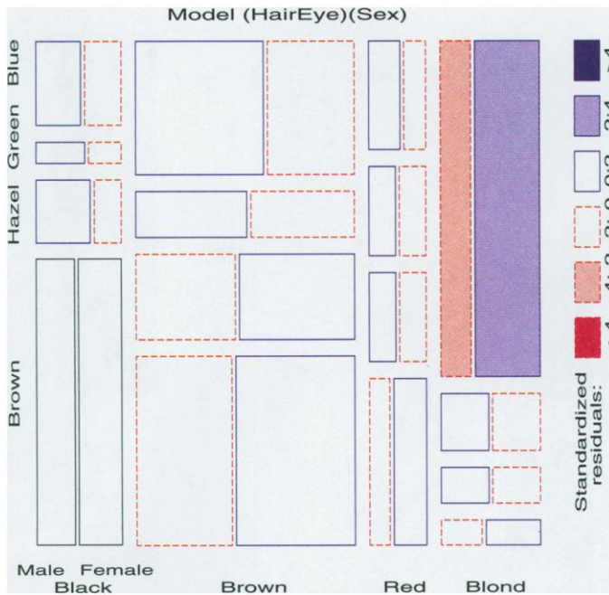
Figure 3. Three-way mosaic display for hair color, eye color, and sex. The categories of sex are crossed with those of hair color, but only the first occurrence is labeled. Residuals from the model of joint independence, [HE][S] are shown by shading. The only lack of fit is an overabundance of females among blue-eyed blonds.
