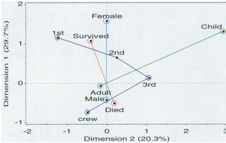
Figure 10. Titanic data: MCA analysis
