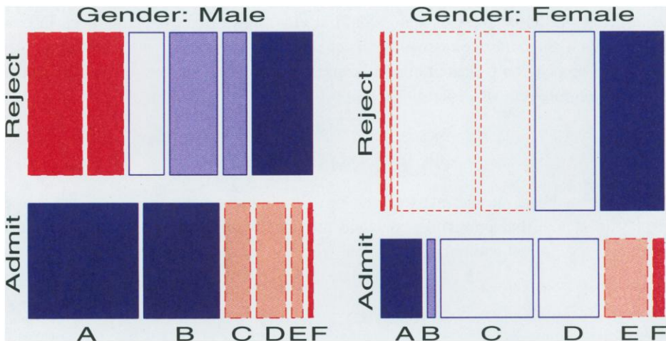
Figure 15. Mosaic cplot of Berkeley admissions, given Gender. Each panel shows the partial relation, fitting a model of independence between Admission and Department.
