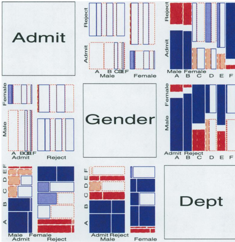
Figure 12. Conditional mosaic matrix of Berkeley admissions. Each panel shows the conditional relation, fitting a model of conditional independence between the row and column variable, controlling for other variable(s).
