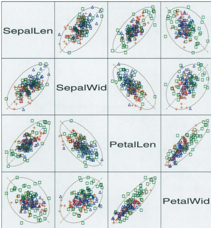
Figure 13. Conditional scatterplot matrix for Iris data. Plot symbols indicate species: Setosa ( \Delta ), Versicolour (+), Virginica ( \square ).
